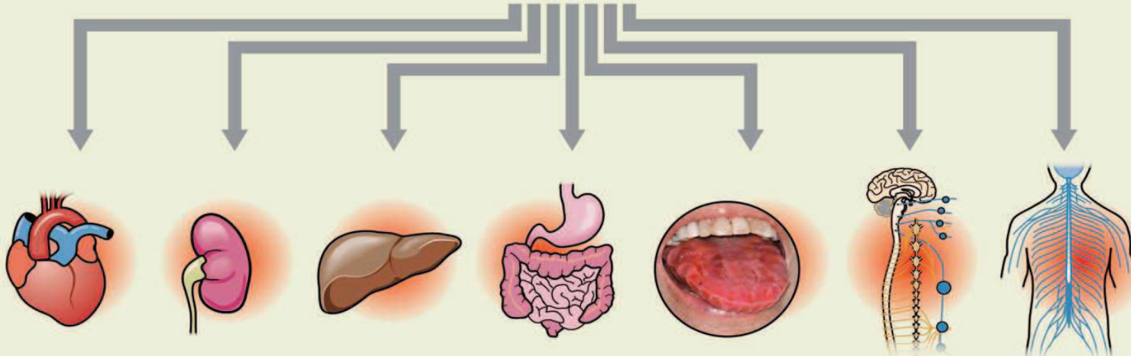
Misfolded monoclonal light chain
