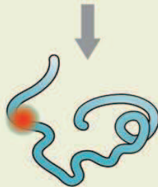
Misfolded monoclonal light chain
